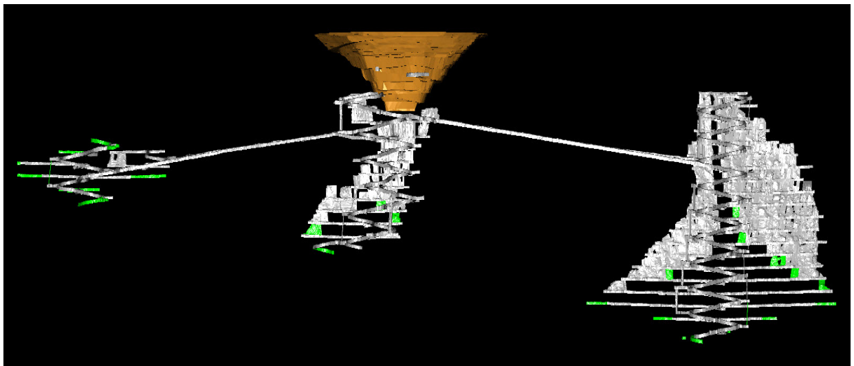
green indicates new developments - stopes are displayed only after reconciliation
